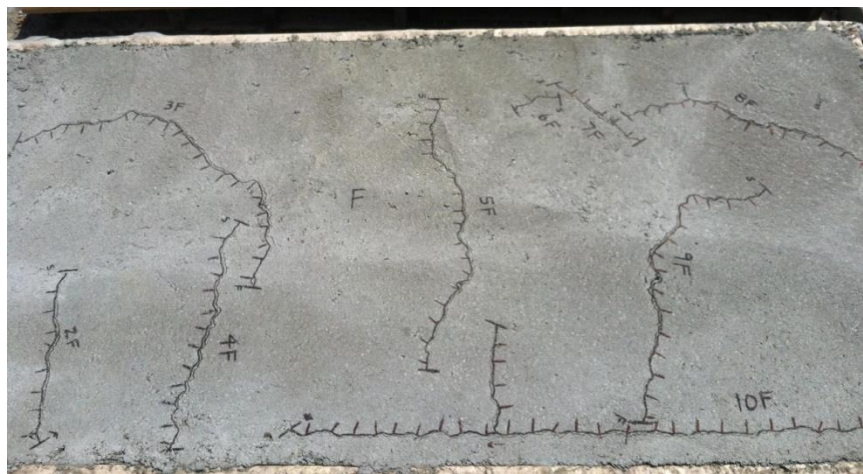
Figure 4.14 Slab Cracks Mapped 24 Hours After Casting
