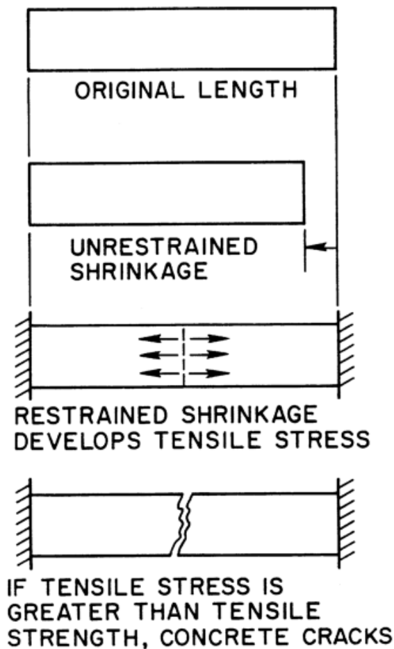
Figure 2.5 Concrete Cracking Due to Drying Shrinkage (ACI, 2001)
